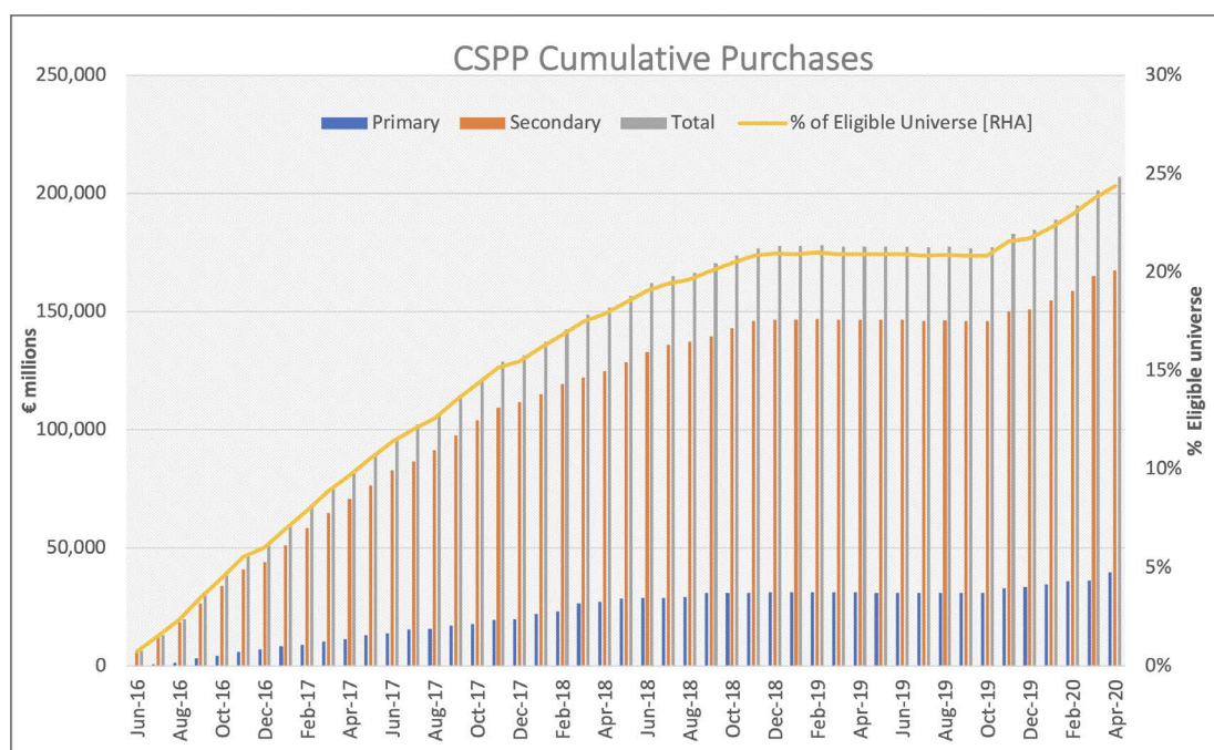
Figure 12: ECB CSPP
